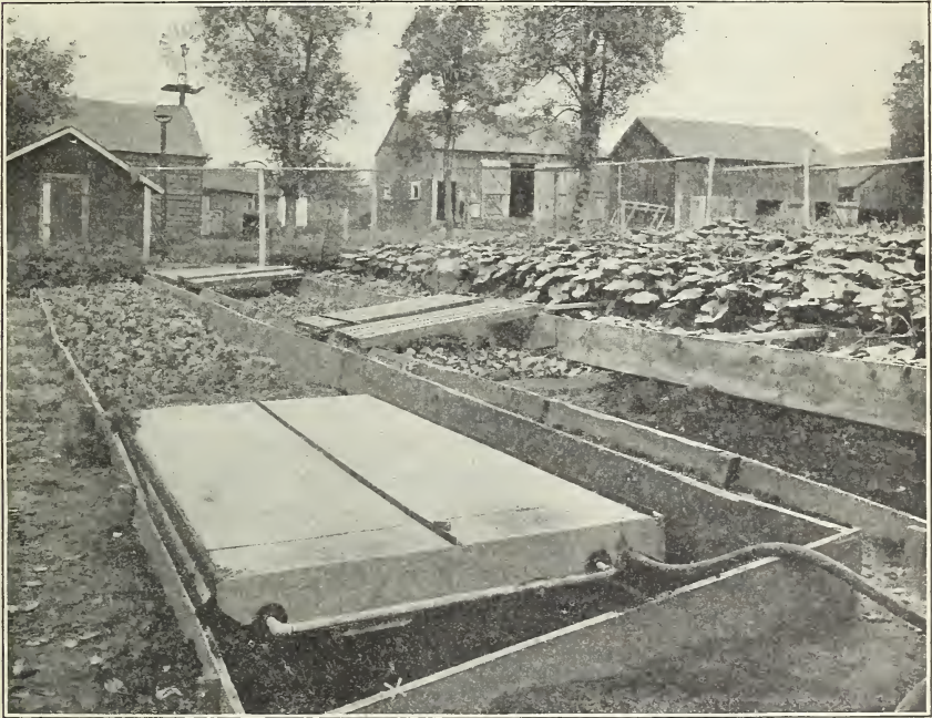
FIG. 5.—Apparatus for steam sterilizing soil by the inverted-pan method.
